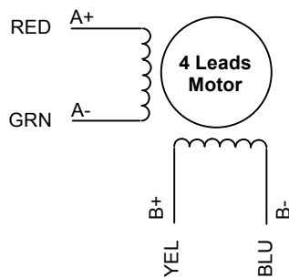
Motor Connection
